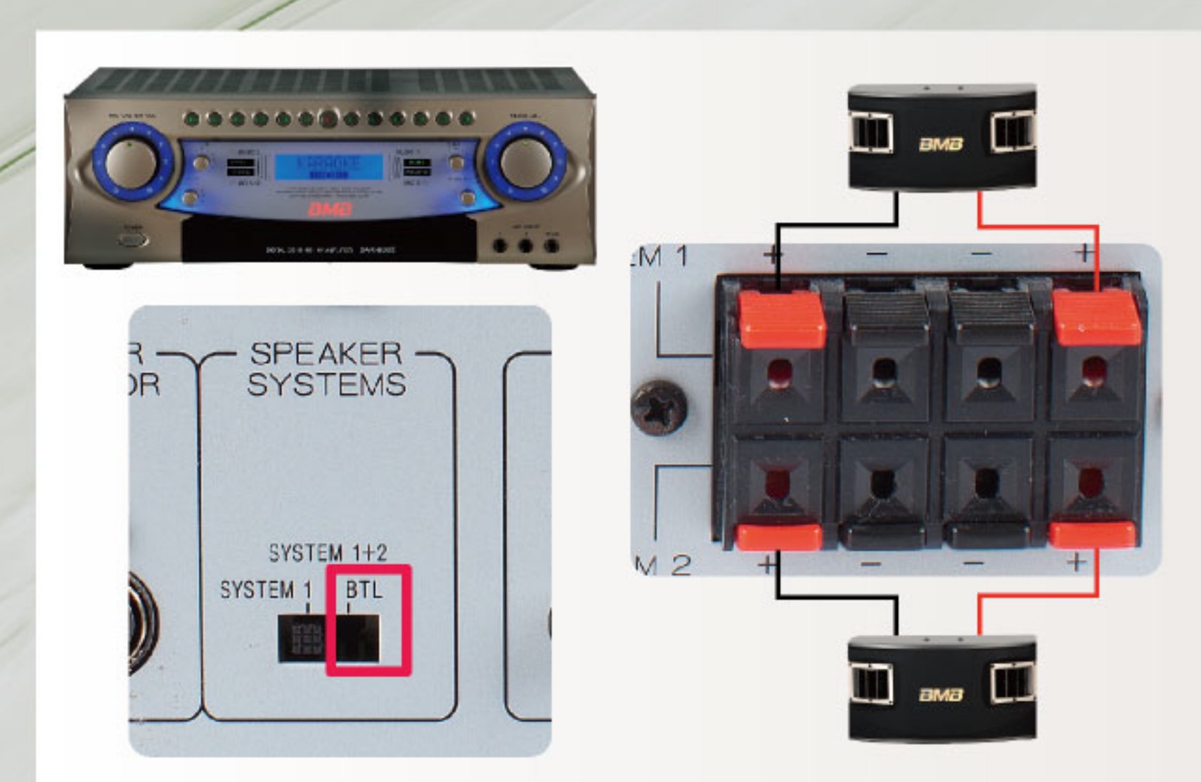
How to connect (360Wx2CH Mode (BTL Mode) )
