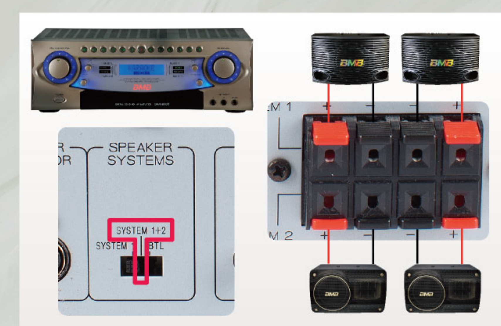
How to connect (150Wx4CH Mode)
