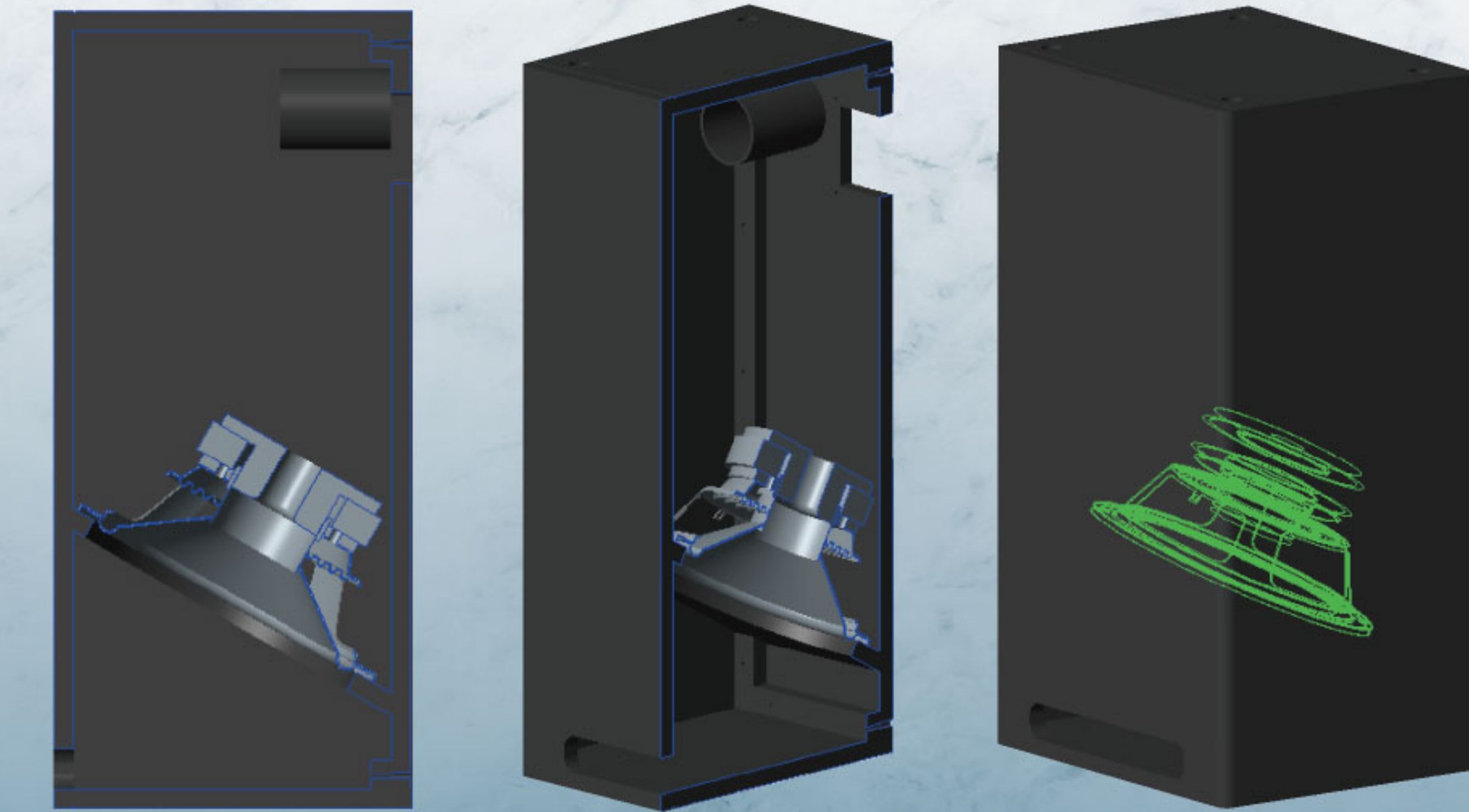
■ SUBWOOFER STRUCTURE Double voice coil system
